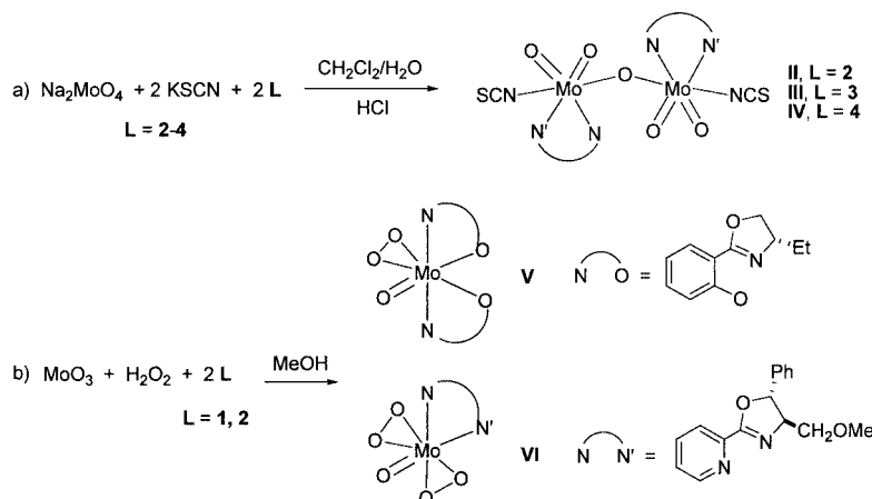
Scheme 1. Synthesis of dioxo(μ-oxo) dimetallic ( II–IV ) (a) and oxo(peroxo) monometallic ( V and VI ) (b) molybdenum(VI) complexes
