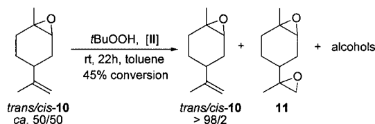
Scheme 3. trans/cis -Limonene oxide ( 10 ) epoxidation catalysed by II using t BuOOH as an oxidant; olefin/ t BuOOH/Mo = 40:60:1
