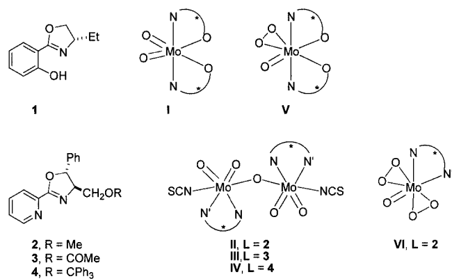
Figure 1. Oxazoline chiral ligands 1–4 and oxomolybdenum complexes I–VI
