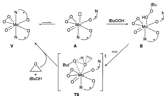
Scheme 4. Mechanistic proposal for olefin epoxidation catalysed by seven-coordinate molybdenum species containing hemilabile ligands
