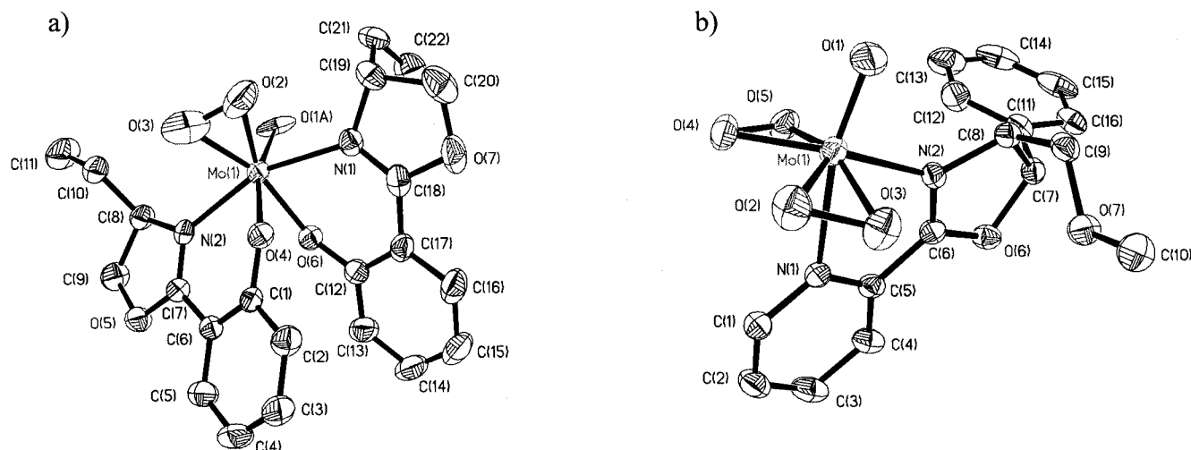
Figure 3. ORTEP diagrams of the molecular structures of V (a) and VI (b); hydrogen atoms are omitted for clarity
