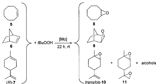
Scheme 2. Cyclooctene ( 5 ), norbornene ( 6 ) and ( R )-limonene ( 7 ) epoxidation catalysed by I , II , V and VI using t BuOOH as an oxidant; olefin/ t BuOOH/Mo = 40:60:1
