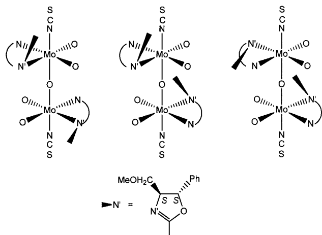
Figure 2. Isomers of dimetallic complex II containing the pure chiral oxazolinylpyridine ligand 2 , with an Mo–O–Mo angle of ca. 180°
